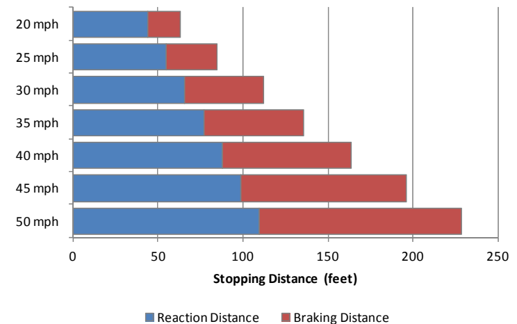
Figure 14: Vehicle Speed and Stopping Distance
